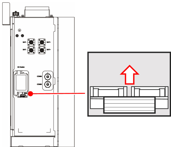
Figure 22: Turning on the DC switch
