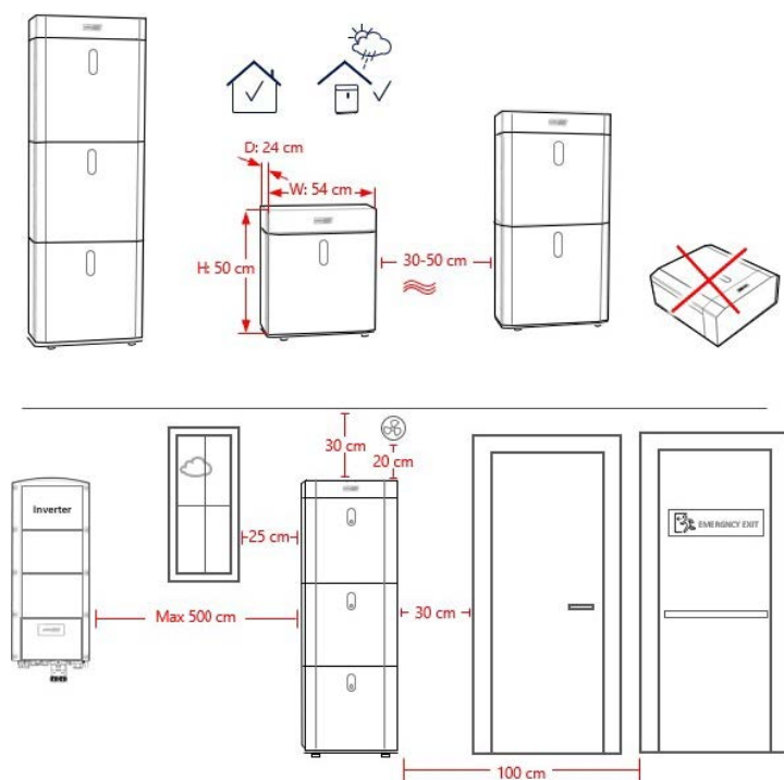
Figure 2: Clearance
