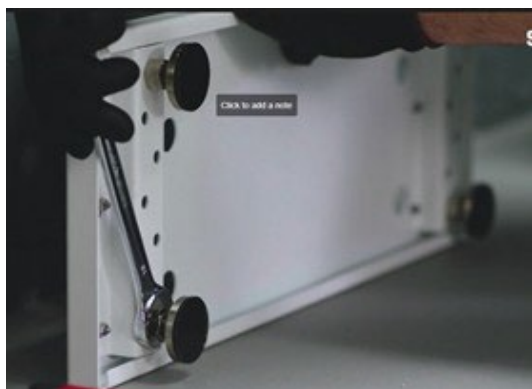
Figure 6: Floor stand—tightening the nut
